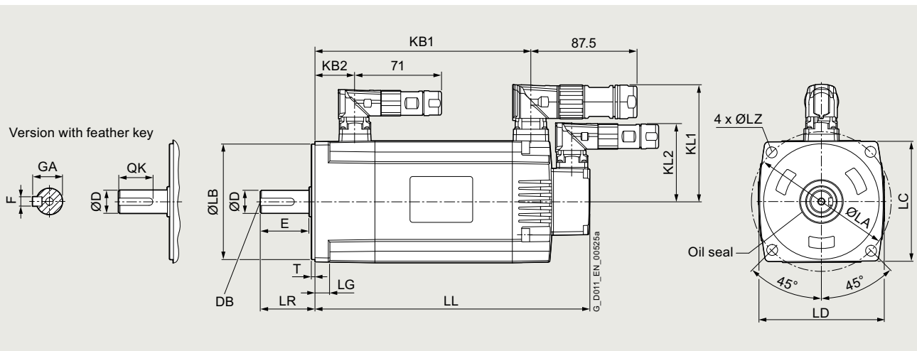
SIMOTICS S-1FL6 Low Inertia servomotor, shaft height 50
